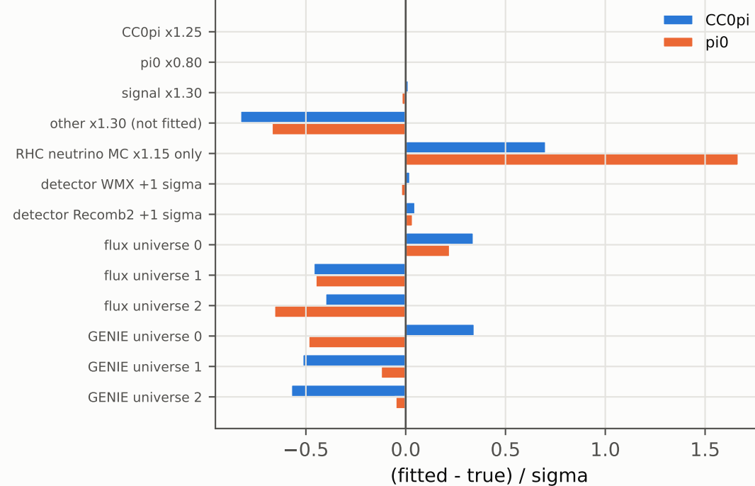
2D: Asimov injections (two-parameter model)
