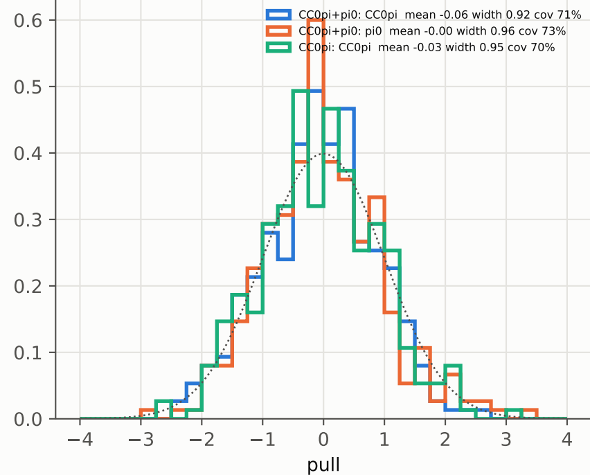
2D: toy pulls (300 toys)
