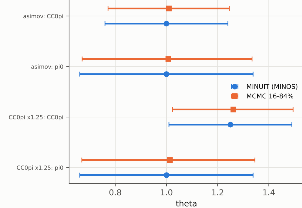
2D: profile likelihood vs MCMC
