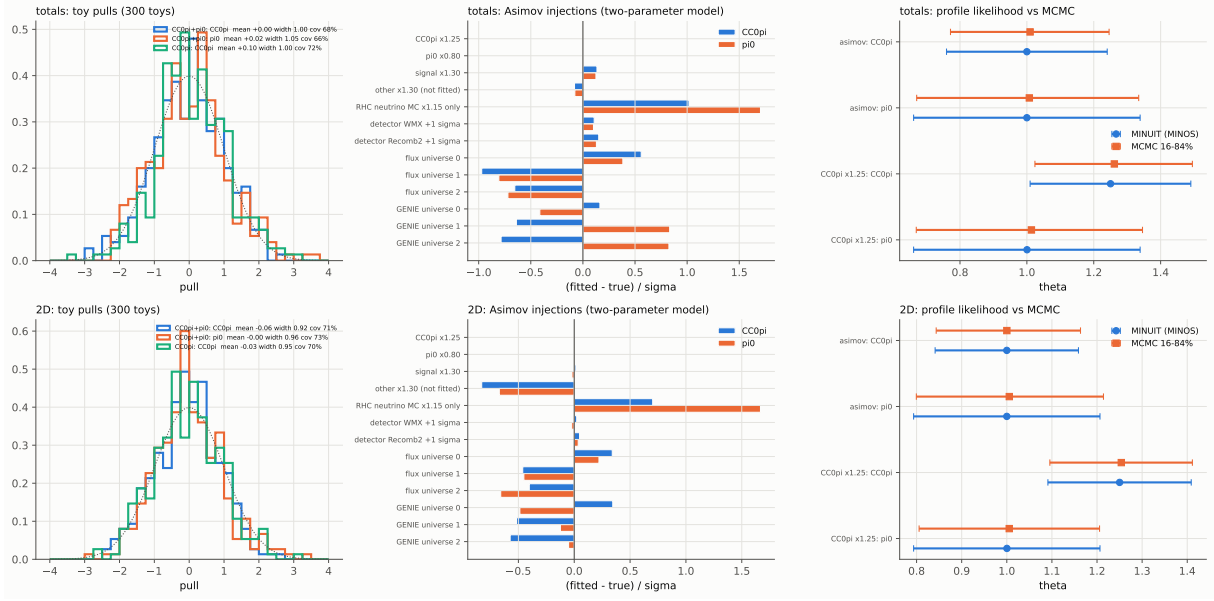
Figure 11: Validation of the background fit on simulation, for the totals-only fit (top) and the two-dimensional fit (bottom): pull distributions from toy ensembles, recovery of injected normalisation shifts, and the profile-likelihood interval against the Markov-chain posterior.
