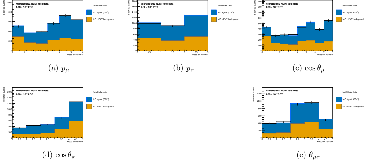
Figure 13: Stage 1, combined: selected reconstructed spectra in the combined configuration.
