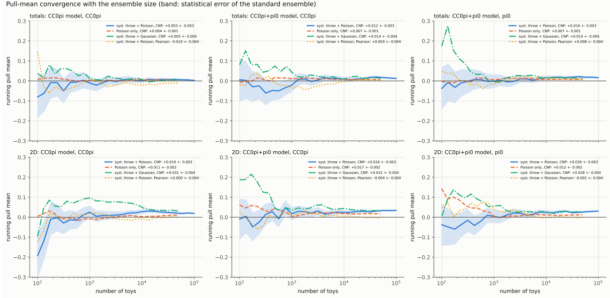
Figure 12: Running pull mean against the ensemble size for each model and parameter; band: statistical error of the standard ensemble. The ensemble thrown with statistical fluctuations only, and no systematic variation, has narrower pulls as expected.
