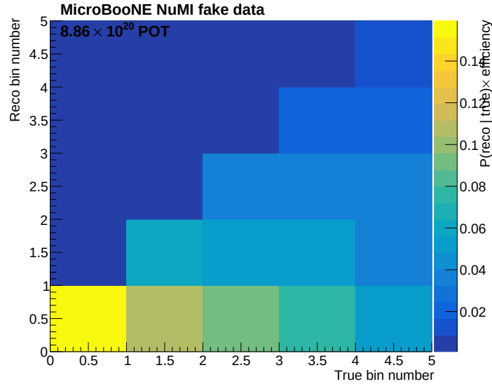
Figure 15: Smearceptance matrix of the rejected five-bin p_\pi scheme (FHC, analysis sample): reconstructed events pile into the lowest bin from every true bin, the diagnostic that motivated the merged regions of §7.2.5; the three-region response of the results is in the analysis note.
