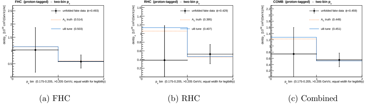
Figure 4: The two-bin p_\pi cross section on the proton-tagged CC1mu1pi1p selection, the graphical form of Tab. 10. The first bin is that of the inclusive result of Fig. 2, and the second is the union of the two upper inclusive regions, since three regions fail the 0.50 criterion in the proton-tagged analysis sample. The bins are drawn equal-width.
