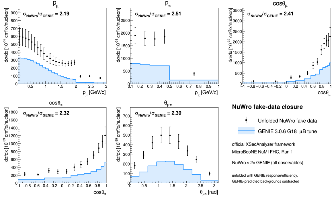
Figure 32: NuWro fake-data closure in the official XSECAANALYZER framework. Points: unfolded NuWro fake data; shaded line: GENIE 3.0.6 G18 \mu B tune. The unfolded NuWro result sits a uniform \approx 2\times above the GENIE prediction in all five observables.
