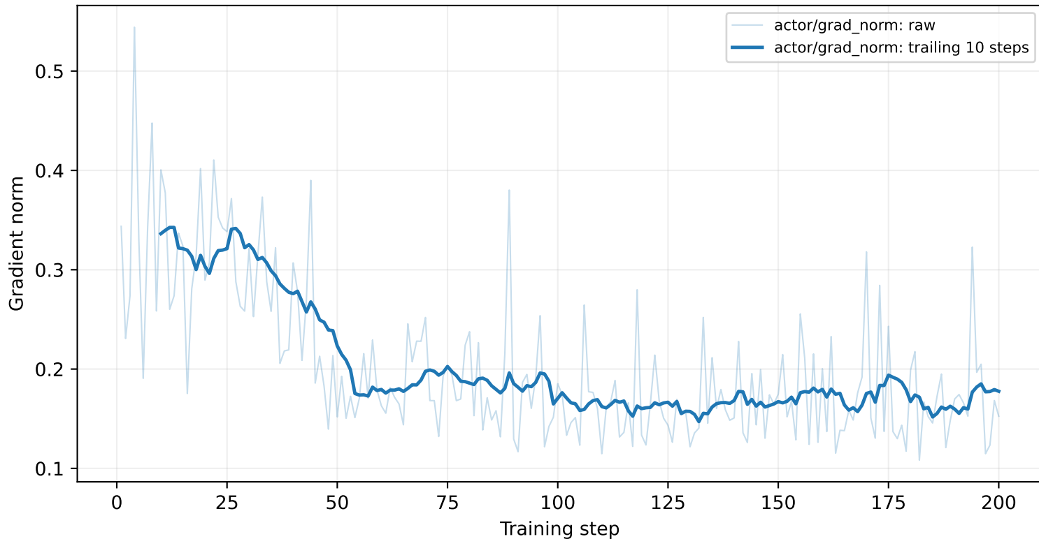
Actor gradient norm
