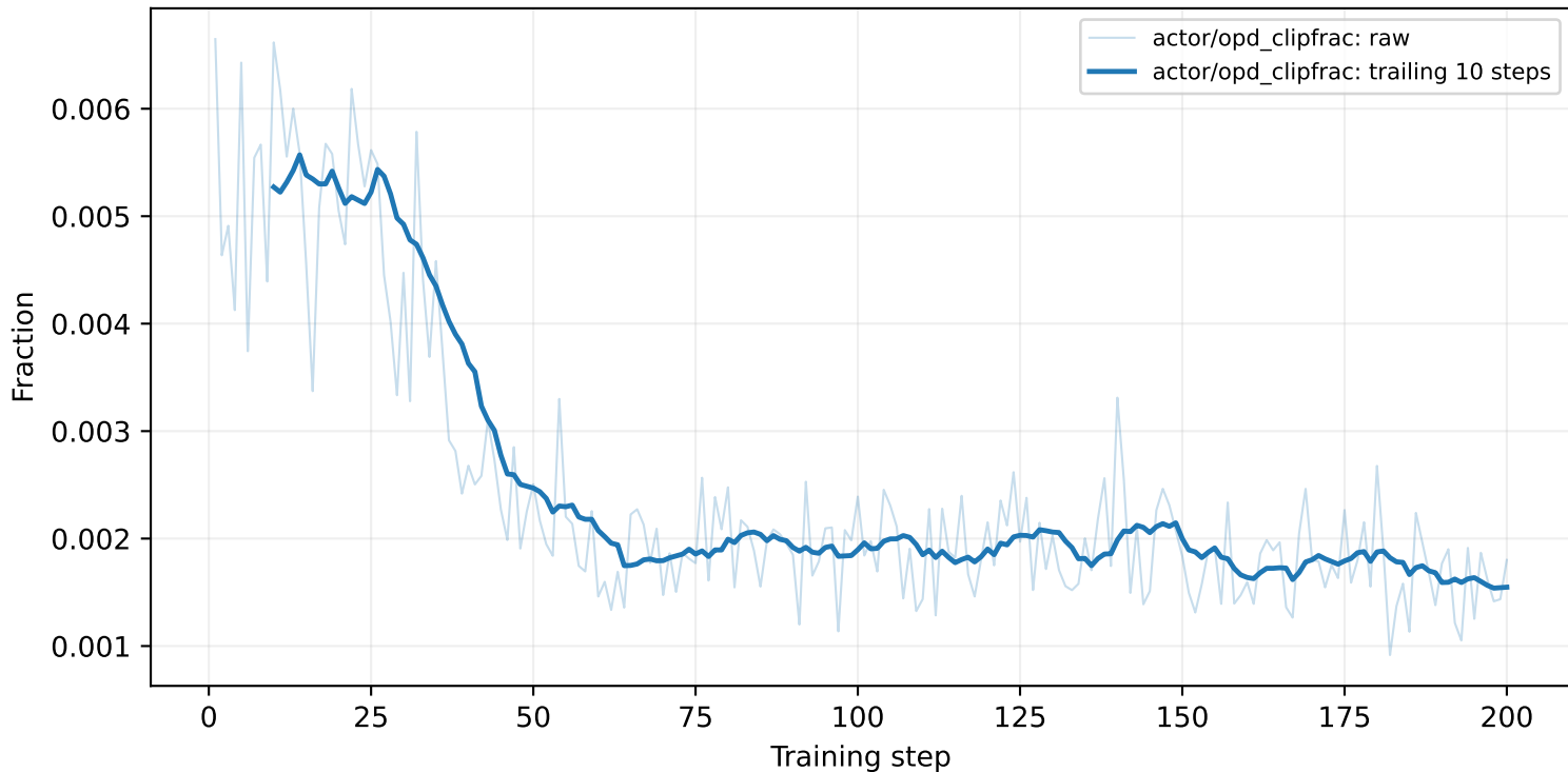
OPD clipping fraction
