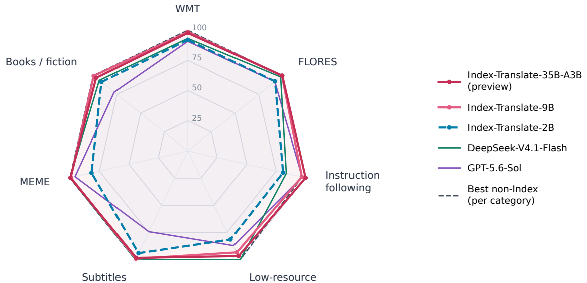
Figure 1: Seven-category text-translation comparison using the online demo 's updated aggregates. Each axis is min-max normalized to 0–100 over all 14 models, including 35B-A3B (preview). Instruction following averages instTrans and IFMT-Bench IFscore; subtitles average OpenSubtitles and MuST-Cinema; books average OPUS-Books and GuoFeng-Webnovel. The gray dashed curve combines the best non-Index score per category.
