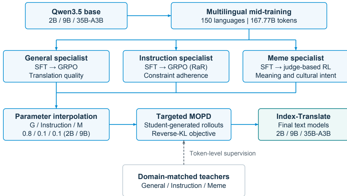
Figure 1: Training overview of the text-model family, including 2B, 9B, and 35B-A3B. General, Instruction, and Meme specialists share a multilingual mid-trained initialization. Parameter interpolation is followed by targeted MOPD, using domain-matched teachers to supervise student-generated rollouts with a reverse-KL objective, to obtain the final models. The displayed interpolation weights apply to the evaluated 2B and 9B models; 35B-A3B results are reported as a preview, with WMT26 pending. Judge-based rewards use RIVAL supervision as described in Section 2.2.
