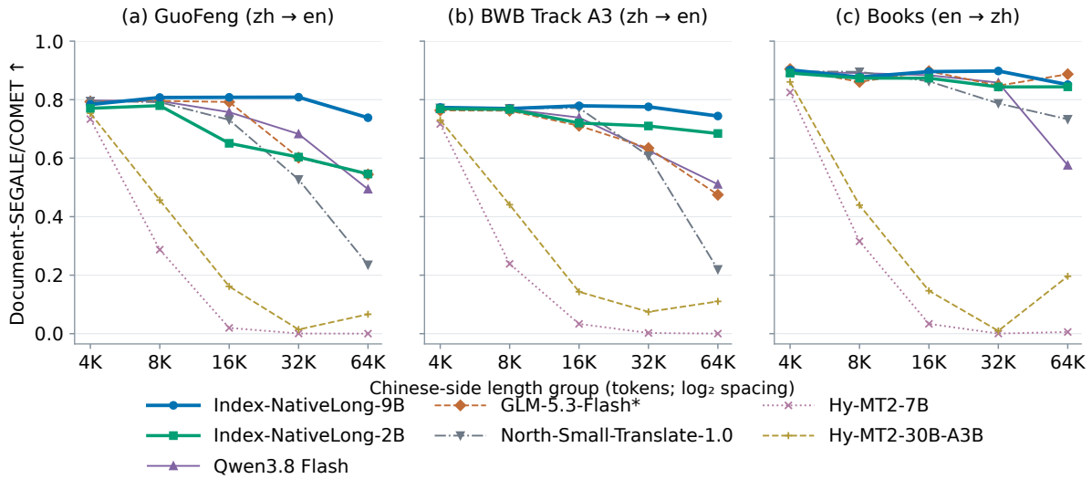
Figure 3: Native long-document translation across Chinese-side length groups, reproducing the point estimates in Table 12. Higher document-SEGALE/COMET is better; unmatched blocks receive zero, so the score reflects coverage as well as translation quality. *GLM’s Books scores average non-refused samples. North uses the experimental context extension described in Section 4.6.
