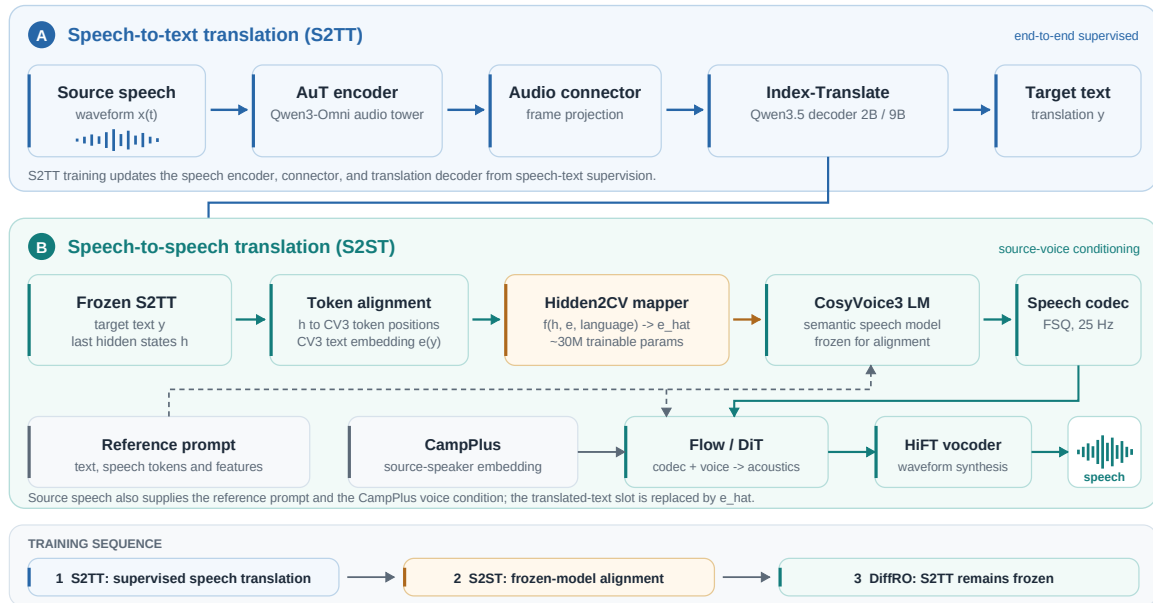
Figure 2: Index-Echo speech-to-text and speech-to-speech architecture. S2ST training aligns the mapper and then applies DiffRO; the S2TT backbone remains frozen throughout.
