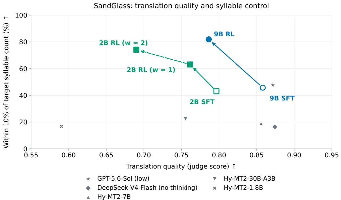
Figure 4: Quality and syllable-control trade-offs on SandGlass. Points reproduce Index-Homura and selected baselines from Table 9; the additional 2B point with syllable-reward weight w = 2 comes from the study in this section. Blue and green denote the 9B and 2B Homura models. Solid arrows connect SFT to RL, and the dashed arrow connects the two 2B reward weights. Both axes favor larger values; arrows show changes between evaluated configurations.
