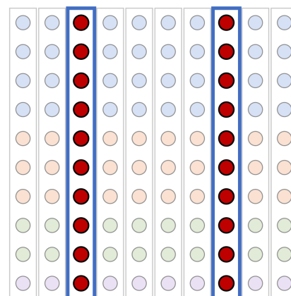
Cluster
