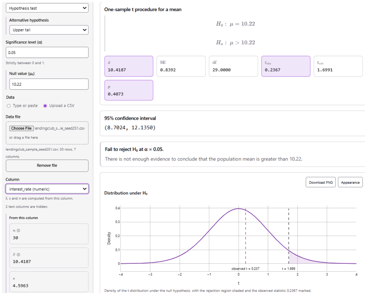
Figure 5. One Sample Tests tool output: SE = 0.8392 , df = 29 , t = 0.2367 , critical value 1.6991, p = 0.4073 , and 95% CI (8.7024, 12.1350). The observed t falls far short of the shaded rejection region.
