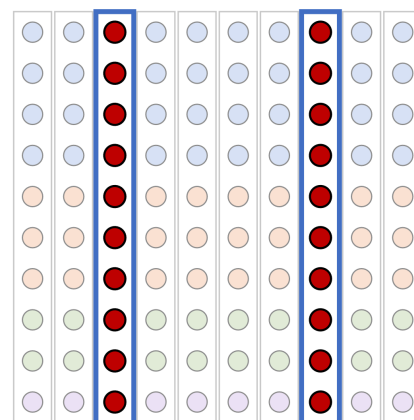
Cluster
