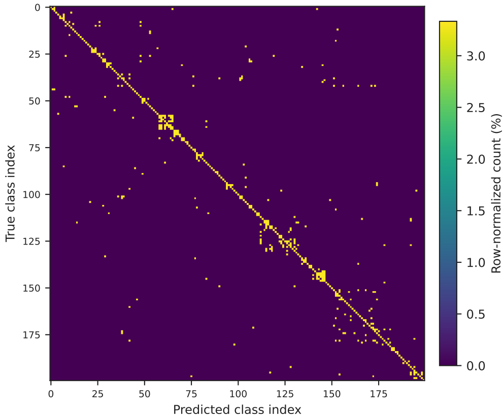
Linear Probe Confusion Matrix
