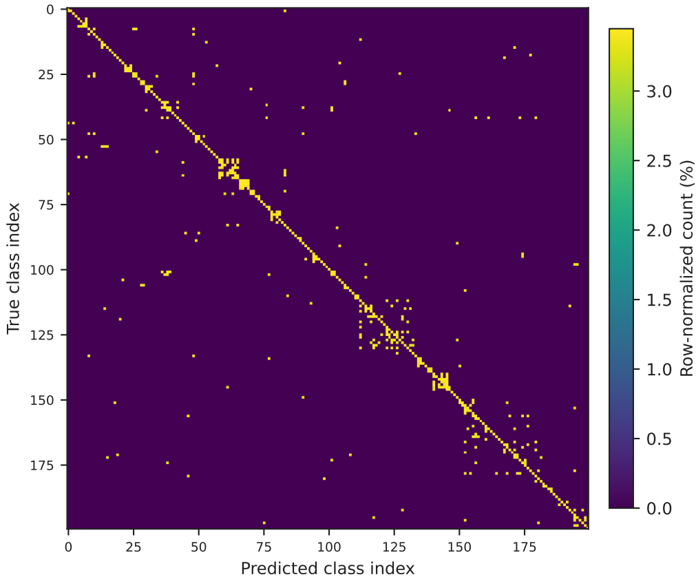
k-NN Confusion Matrix (k=10)
