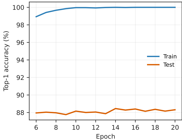
Linear Probe Accuracy
