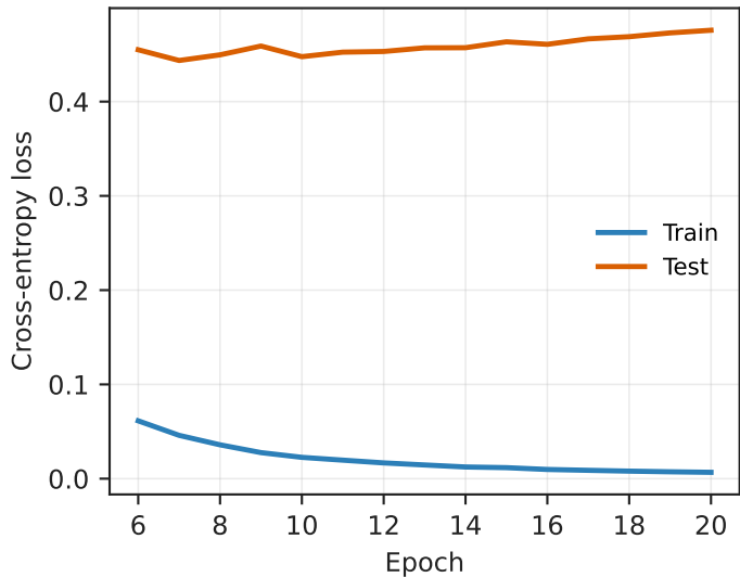
Linear Probe Loss
