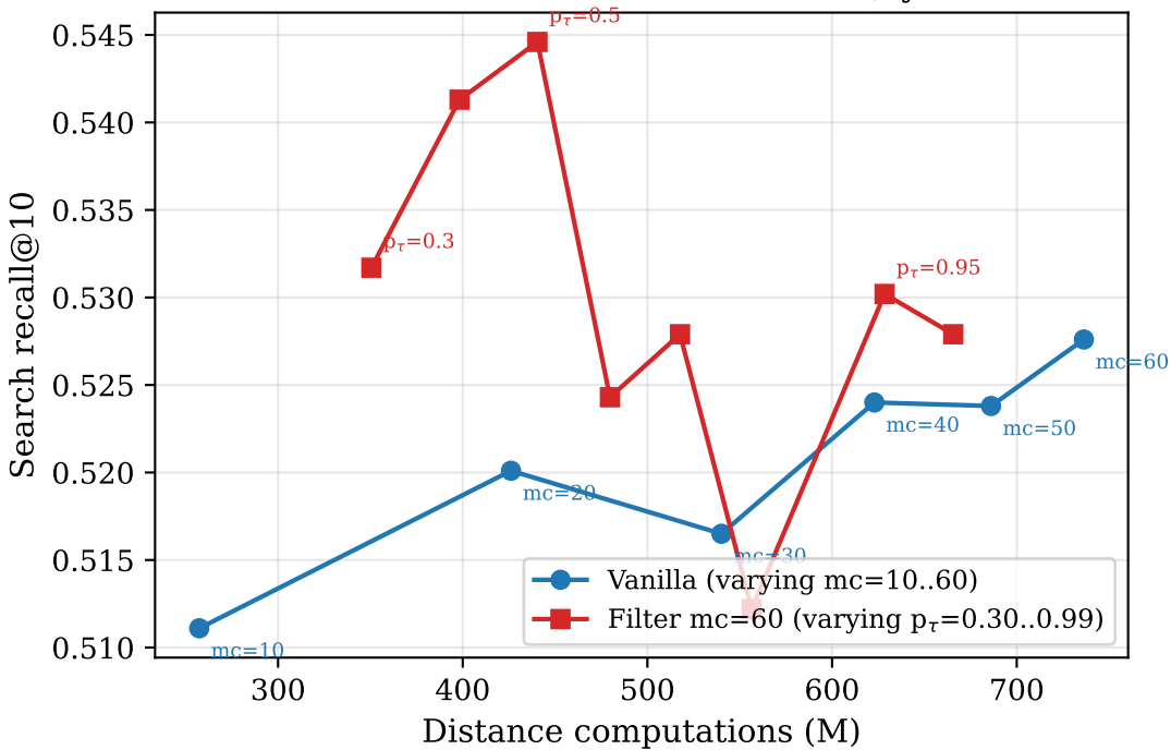
GIST 1M — Search recall vs. construction cost (PyNNDescent, m=16)
