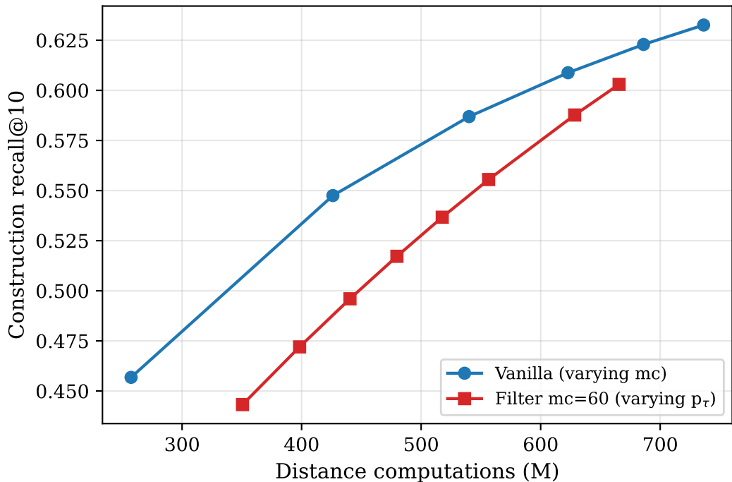
GIST 1M — Construction recall vs. cost (PyNNDescent, m=16)
