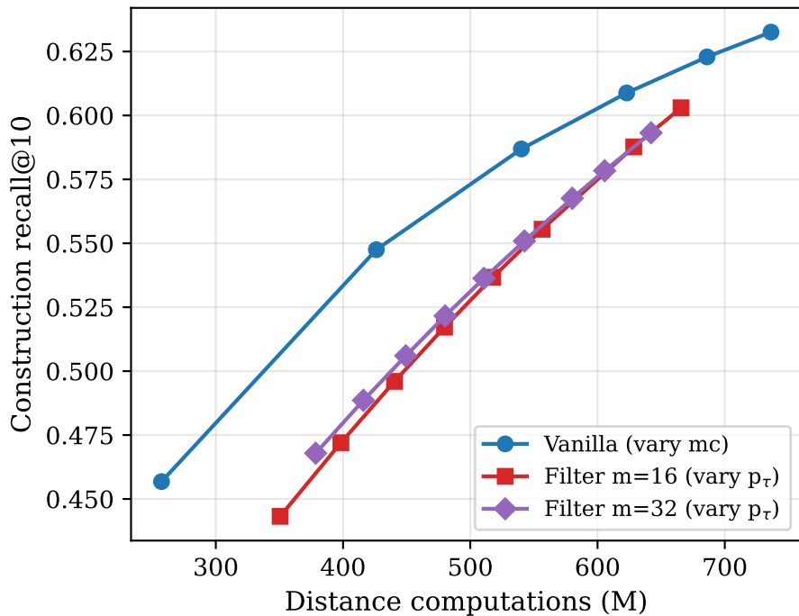
Construction recall vs. cost
