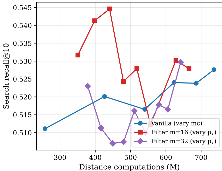
Search recall vs. cost
