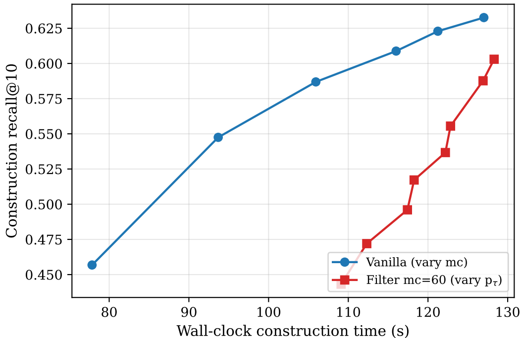
GIST 1M — Construction recall vs. wall-clock (PyNNDescent, m=16)
