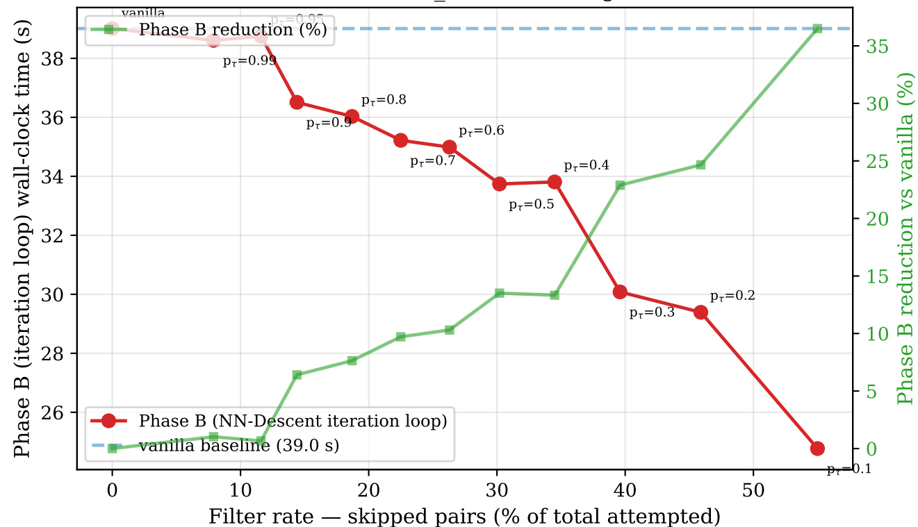
GIST 1M — Phase B time vs filter aggressiveness (mc=10, m=16, tree_init=True, single-thread)
