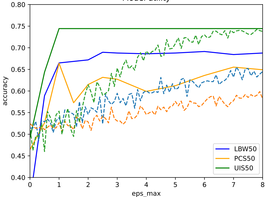
Model utility
