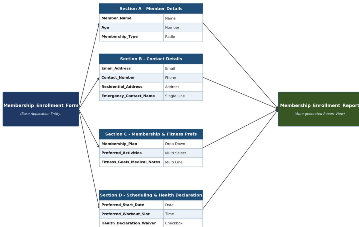
Fig 1. Data Model — Membership_Enrollment_Form and its sectioned fields feeding Membership_Enrollment_Report
