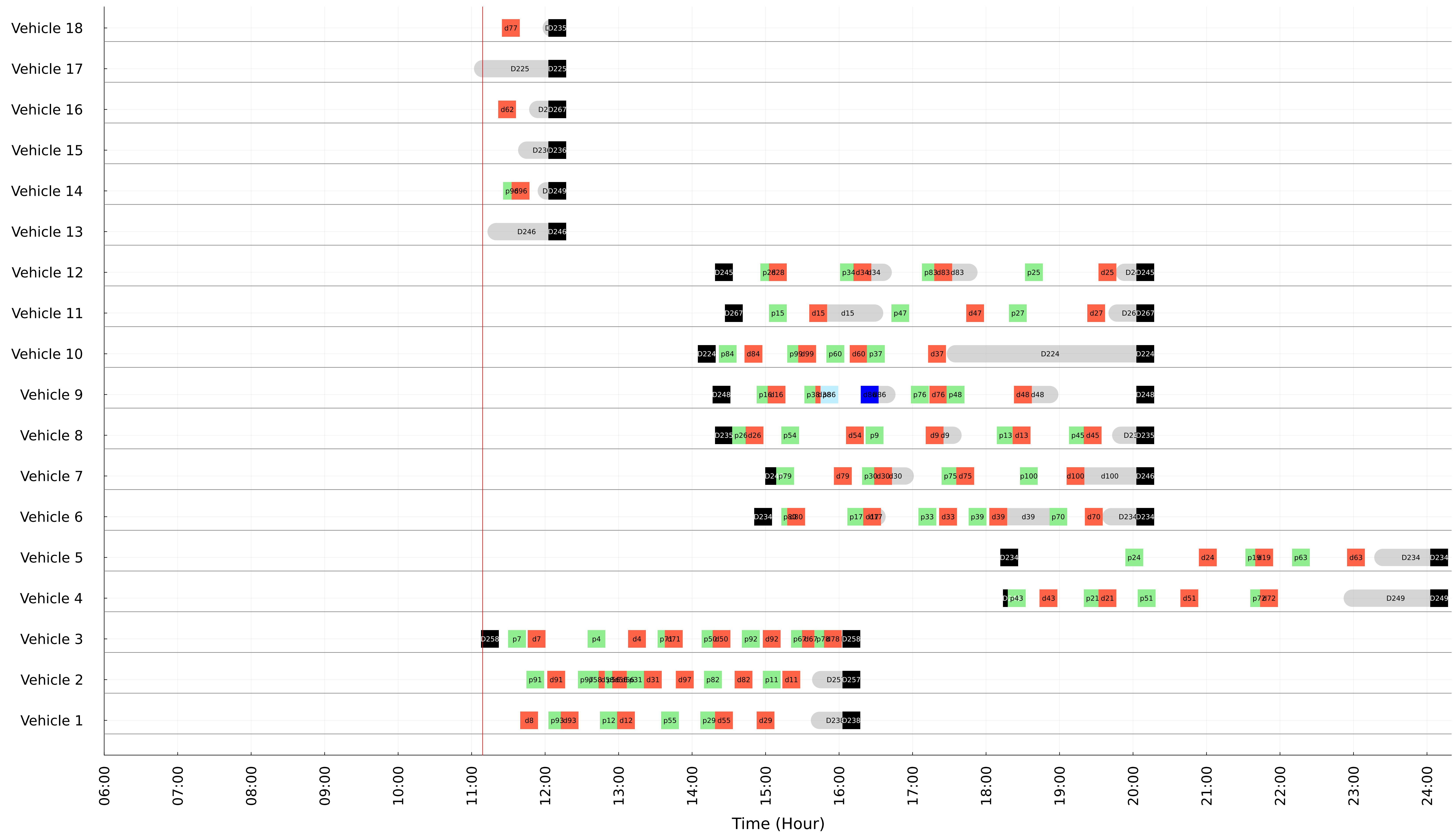
Current Solution, Request: 86, time: 10:59
