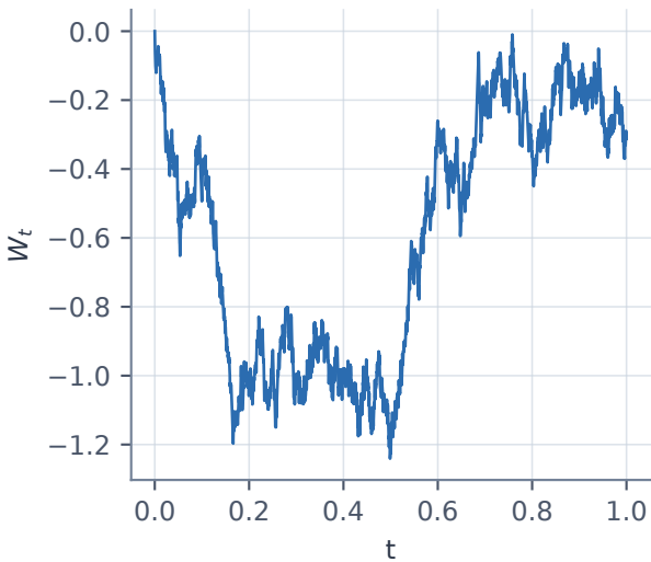
one path
