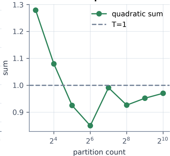
nested partitions
