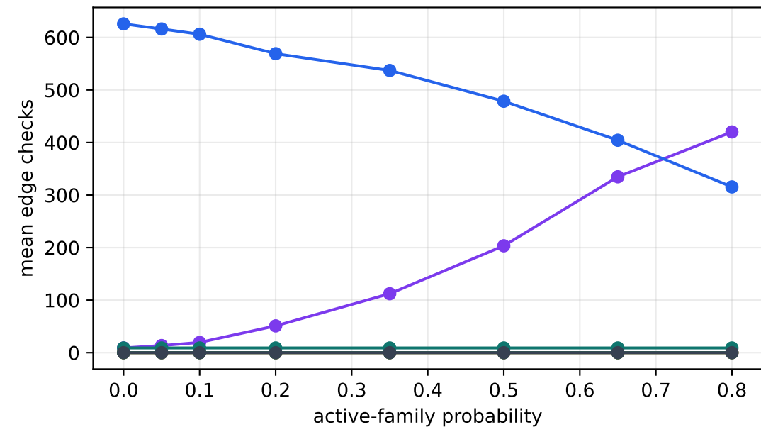
Verifier calls
