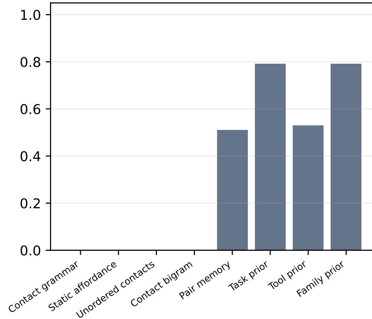
False negatives
