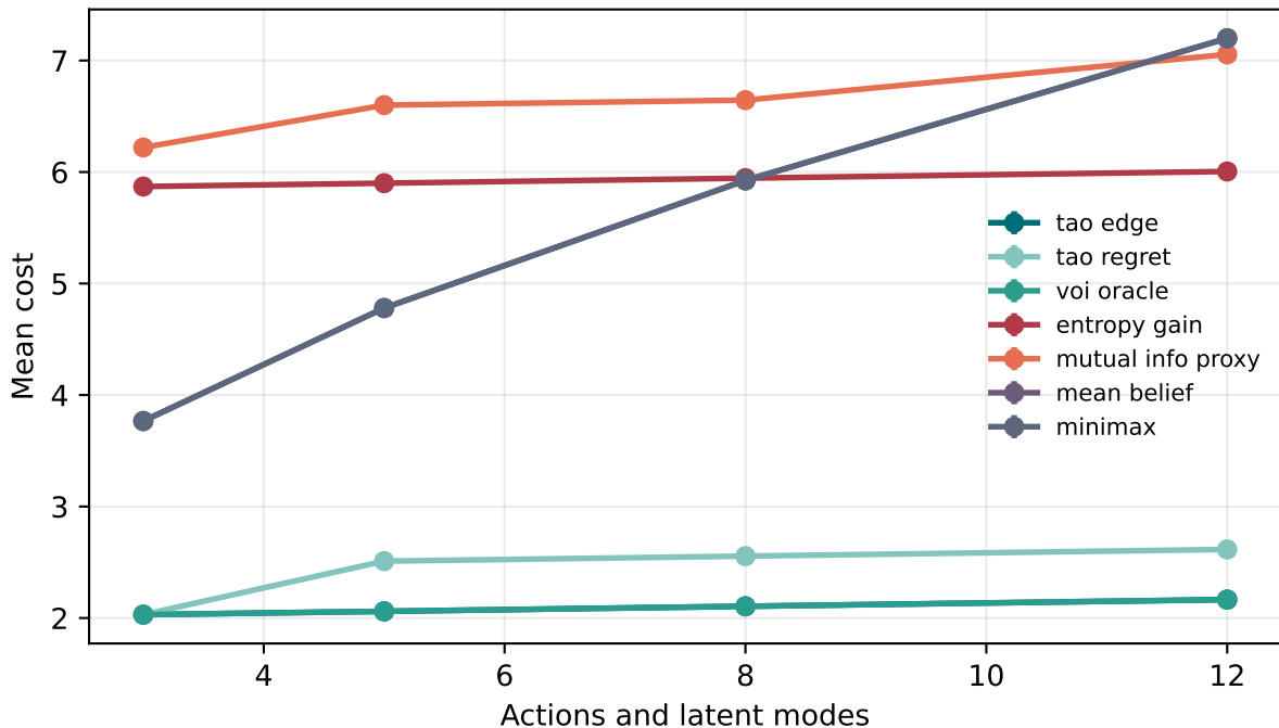
Multi-action inspection, 32 nuisance bits
