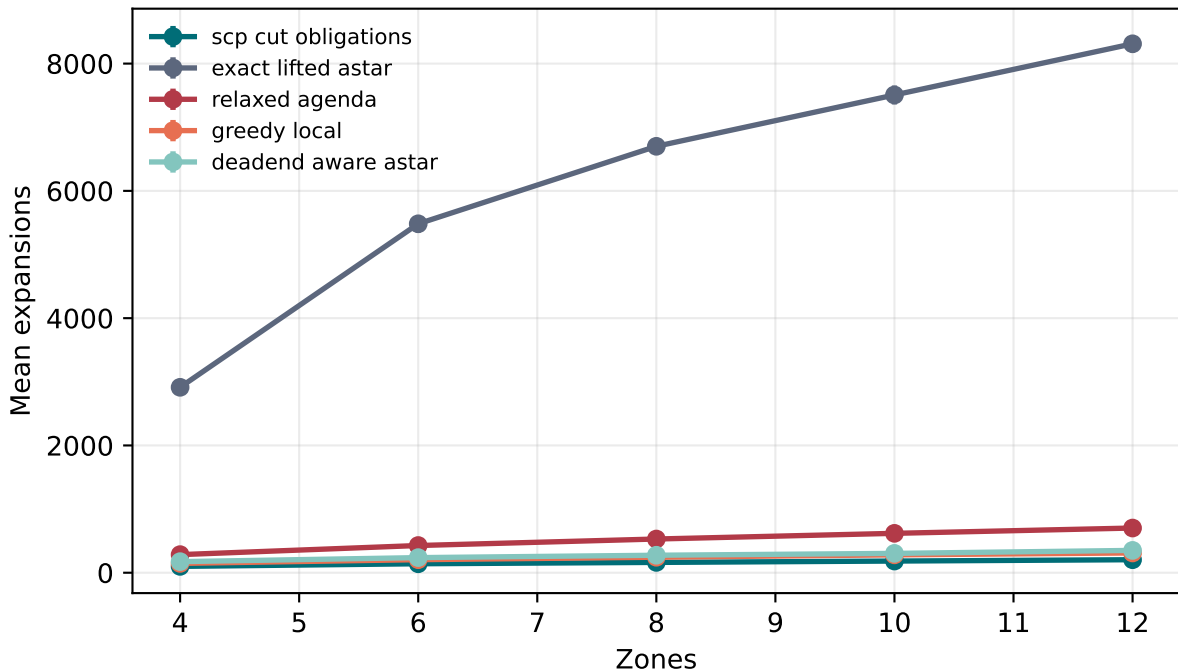
Commitment-zone scaling
