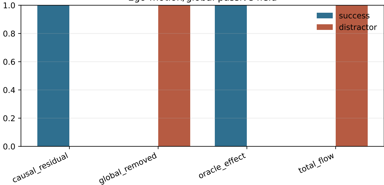
Ego-motion/global passive field
