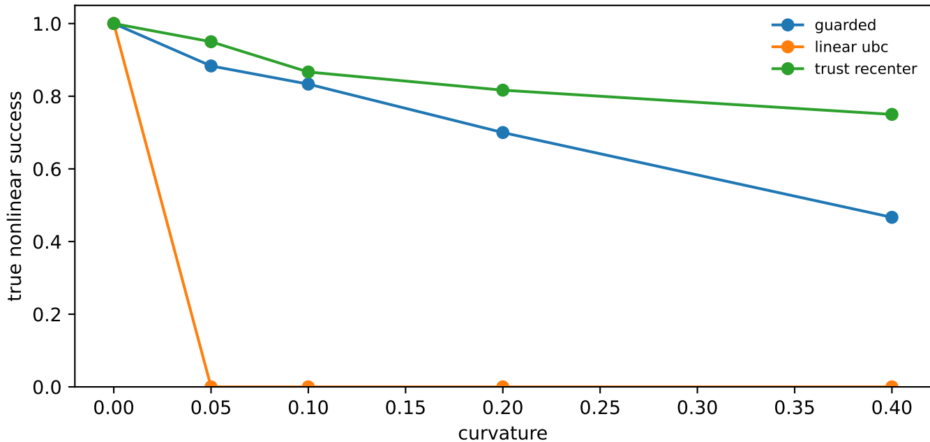
Nonlinear locality stress
