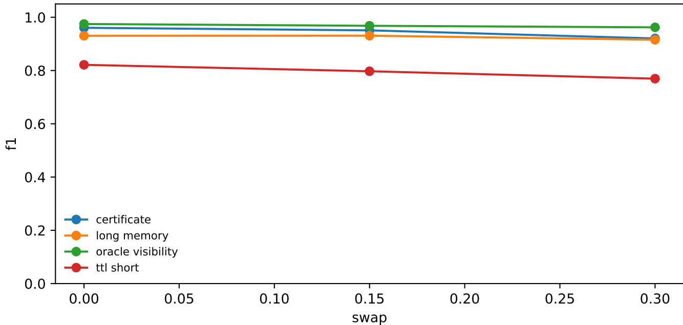
Association ambiguity stress
