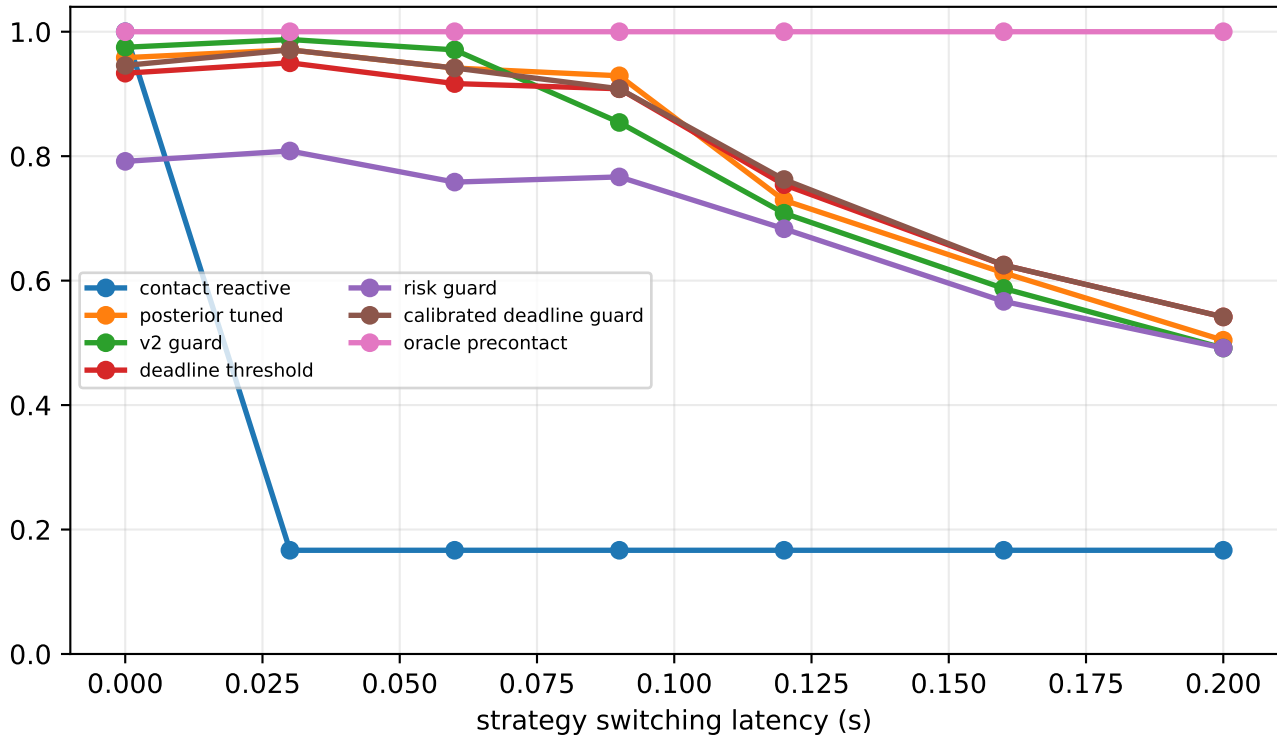
safe success rate
