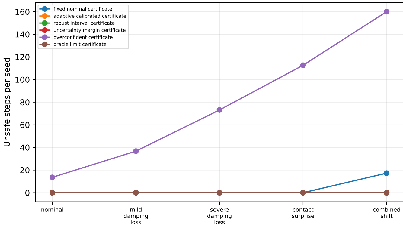
Calibration stress curve
