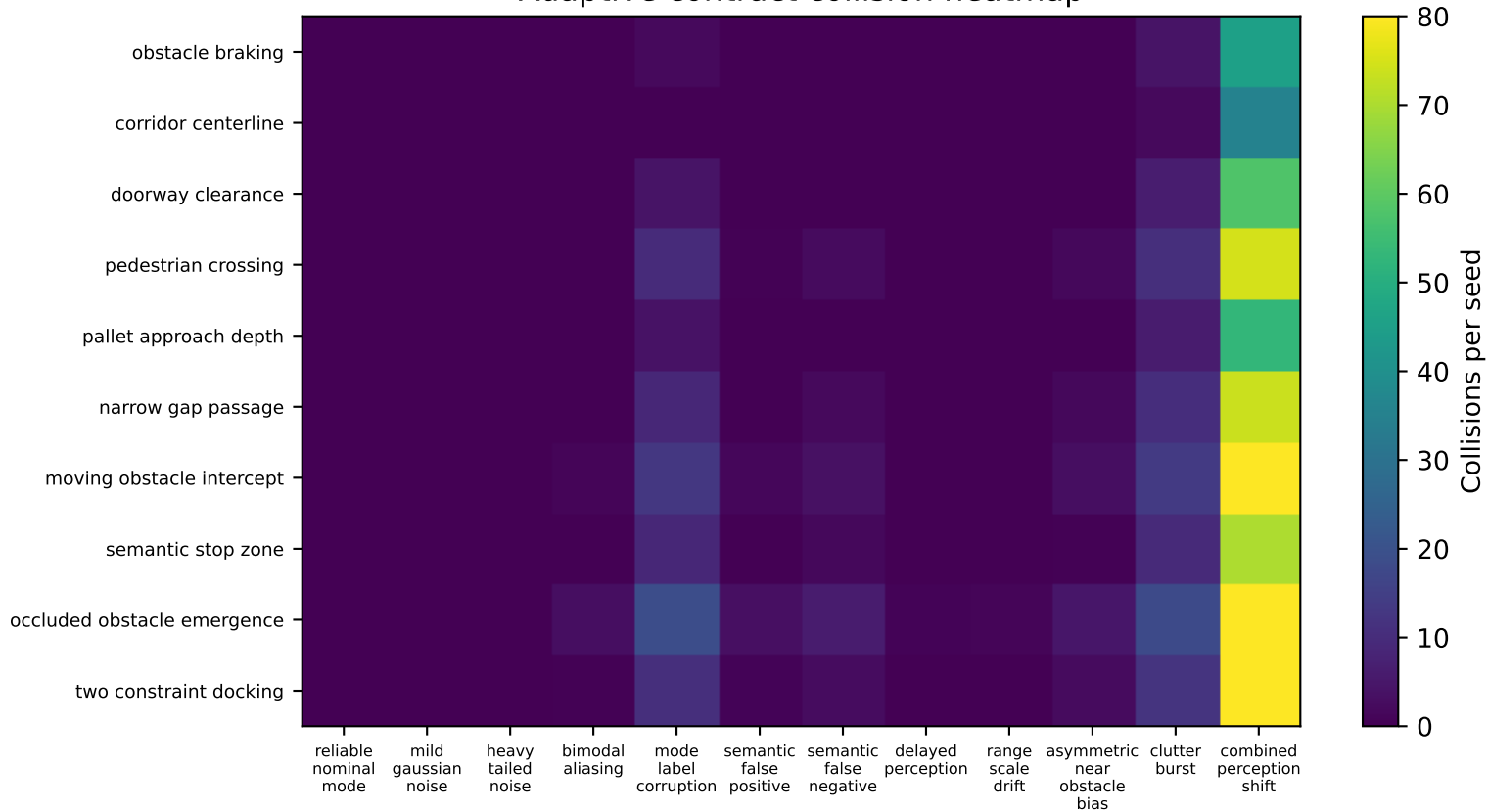
Adaptive contract collision heatmap
