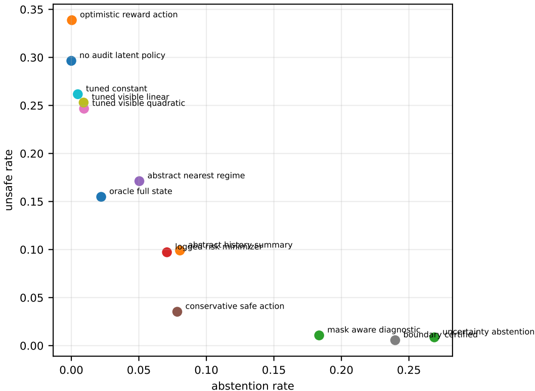
Abstention versus unsafe actions
