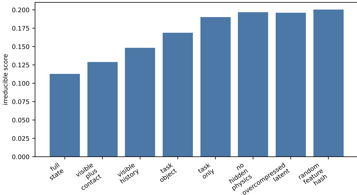
Variable deletion ablation
