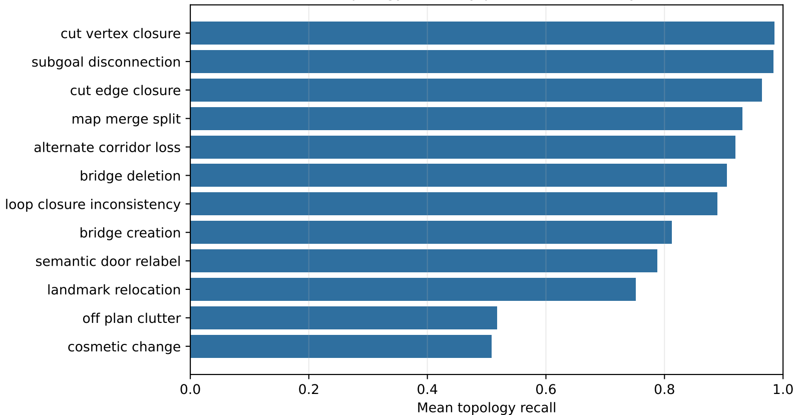
Topology recall by perturbation family
