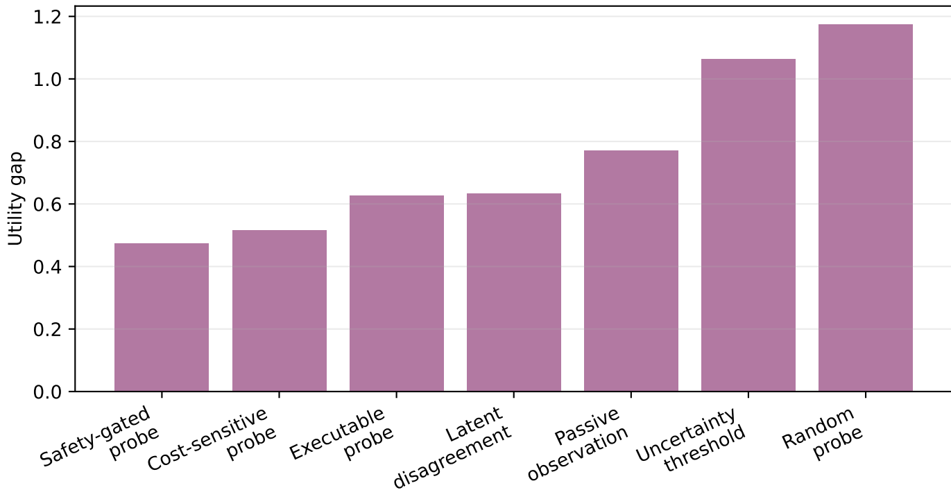
Oracle utility gap by strategy
