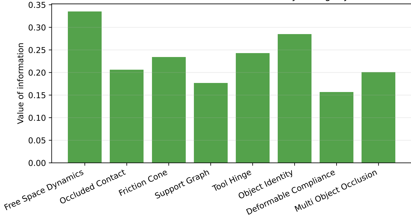
Cost-sensitive value of information by ambiguity
