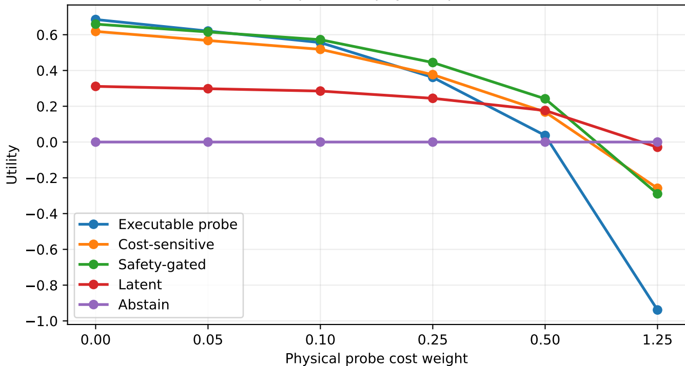
Utility response to physical probe cost
