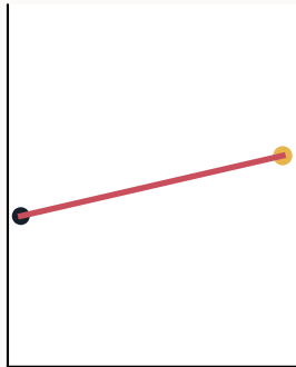
planar pusher
