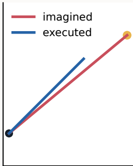
point mass
