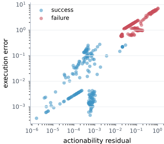
Residual predicts execution gap
