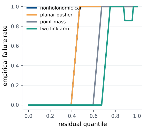
Failure rate rises with residual
