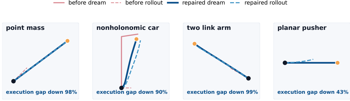
Figure 6: Before/after repair examples. Each card shows a non-executable future, its repaired future, and the rollout recovered from local controls. The repaired trajectories substantially reduce execution mismatch.
