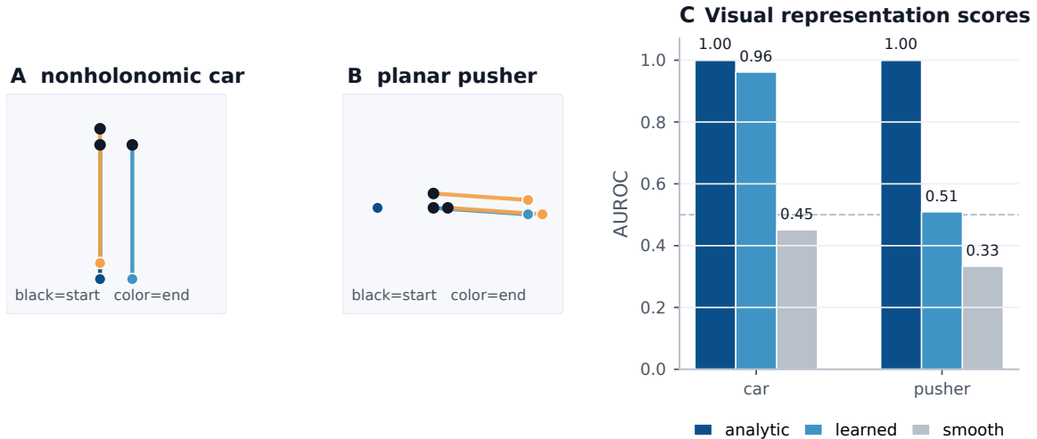
Figure 8: CPU visual/keypoint futures. Actionability remains useful when z is a rendered keypoint representation rather than the raw simulator state. The visual examples and score panel are separated to make the proxy evidence directly inspectable.
