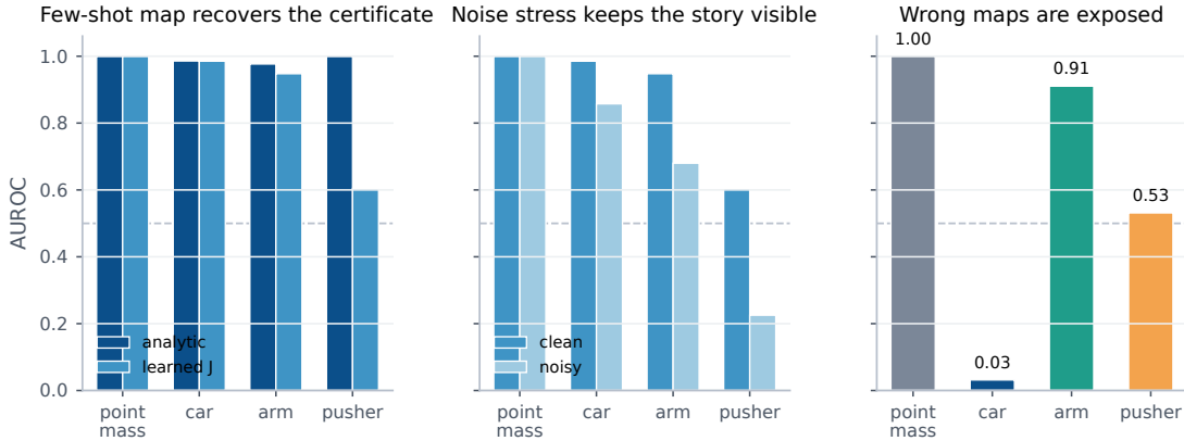
Figure 5: Robustness audit over learned maps. Local Jacobian maps become reliable with modest data in smooth embodiments, remain useful under noise, and expose wrong action maps. The contact pusher remains the hard case because the reachable tangent set changes discontinuously with contact mode.
