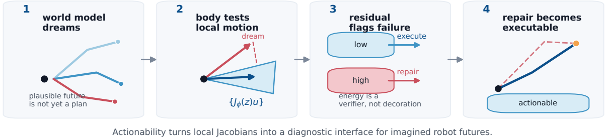
Figure 1: A generated future can be visually plausible while leaving the local action-reachable tangent set. Actionability energy turns an embodiment Jacobian into a diagnostic interface: low-energy futures are executable, while high-energy futures are repaired by composed trajectory inference.
