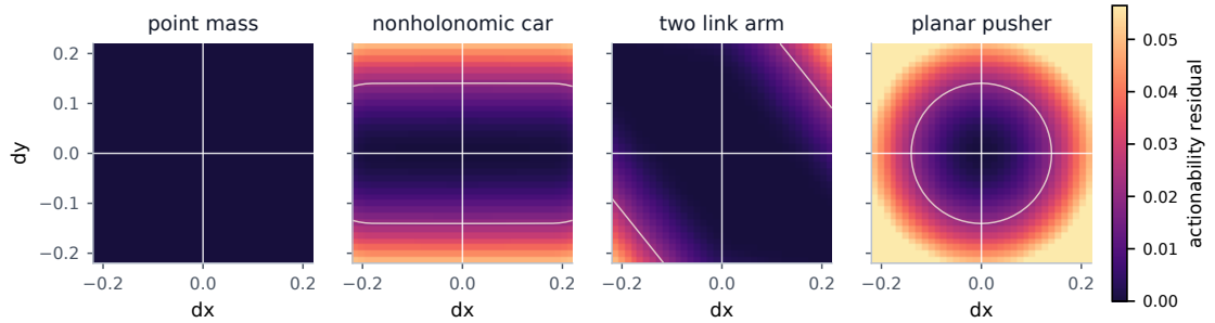
Figure 7: Embodiment swap residual fields. The same representation displacement can be actionable for one body and non-actionable for another. Low residual regions now show the feasible tangent structure without collapsing into unreadable black regions.
