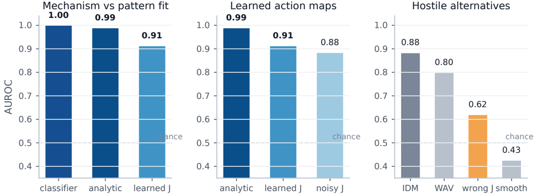
Figure 4: Hostile baseline comparison. Sparse grouped panels separate the learned pattern-fit result from the mechanism-level certificate. Learned-J residuals recover most of the actionability signal, while wrong maps and passive proxies lose the executability distinction.
