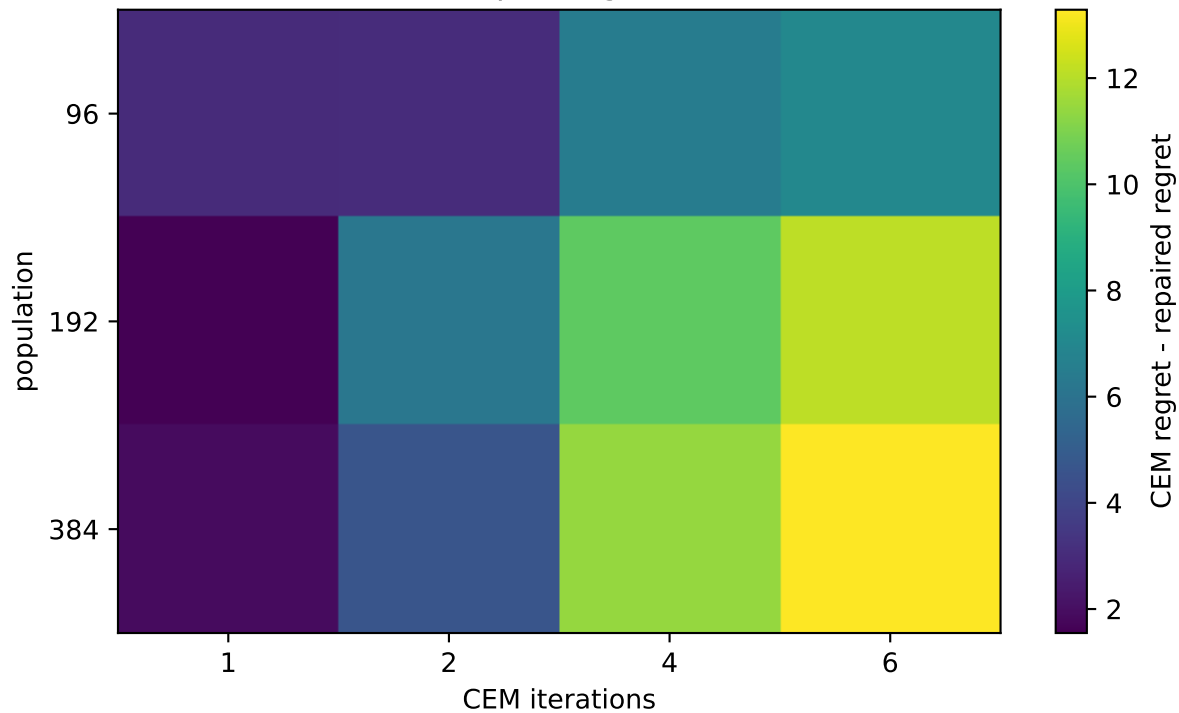
Combined repair regret reduction
