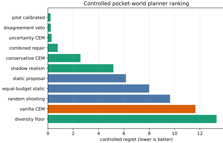
Figure 3: V3 controlled-run planner ranking. Vanilla CEM has substantially higher regret than static proposal baselines, while model-side repairs interrupt the elite-refit failure.
