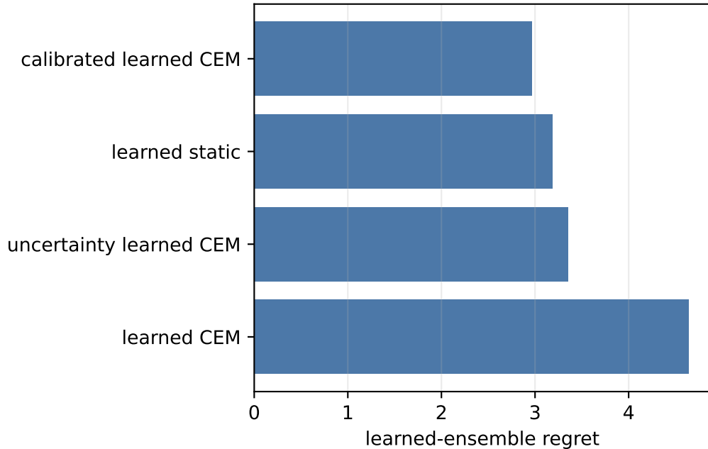
Sparse learned ensemble
