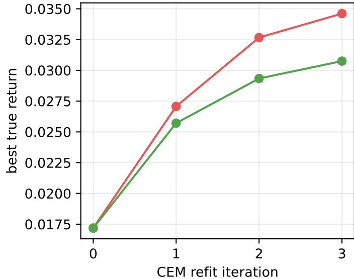
FrozenLake-v1
