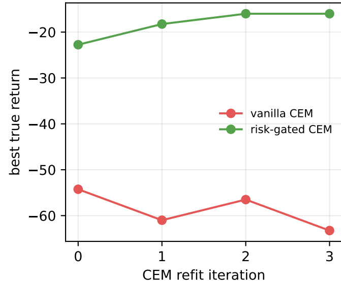
Taxi-v3
