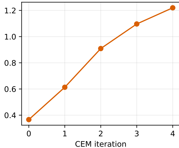
proposal drift
