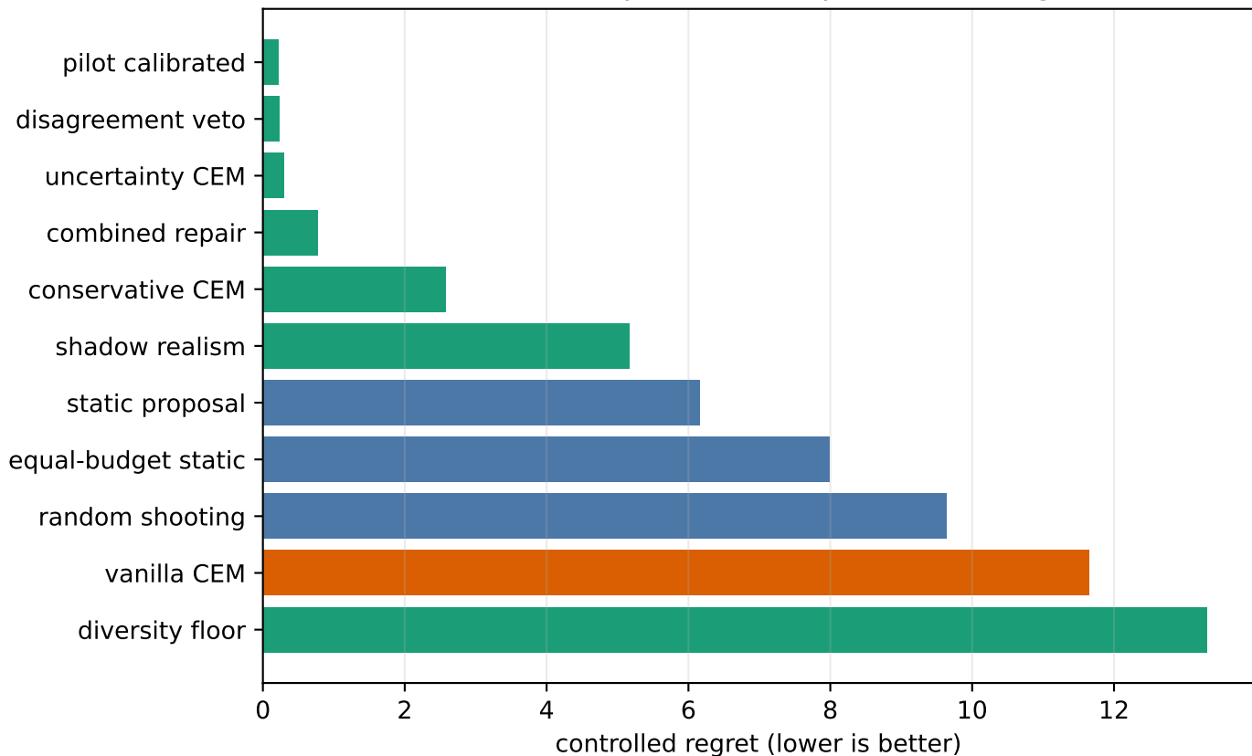
Controlled pocket-world planner ranking
