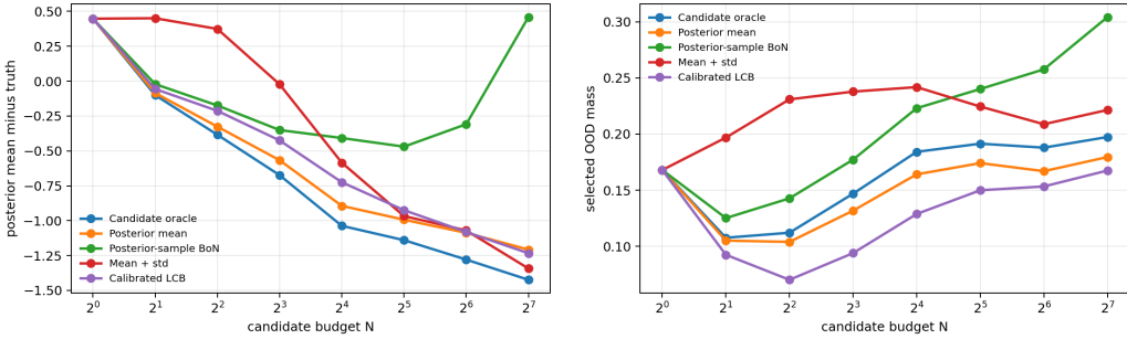
Figure 2: Selected-trajectory diagnostics. Posterior-sampled Best-of-N chooses candidates with higher OOD mass and large sampled-score residuals over the posterior mean.
