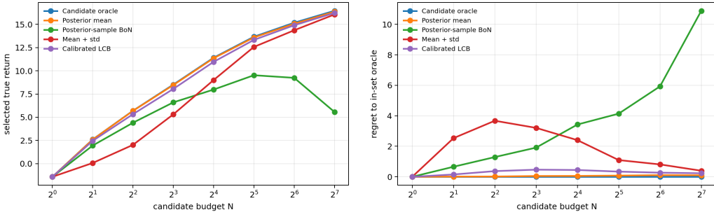
Figure 1: Left: selected true return. Right: regret to the best true-return candidate in the same sampled set. Posterior-sampled Best-of-N degrades at large N despite the candidate set containing strong trajectories.
