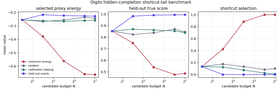
Figure 6: Real-data Digits hidden-completion tier. The prompt is the observed top half of an 8-by-8 handwritten digit from the standard scikit-learn Digits benchmark, and the held-out metric scores the generated bottom half. Minimum energy enters a smooth shortcut tail as N grows; calibrated clipping rejects that tail without reading the held-out pixels.
