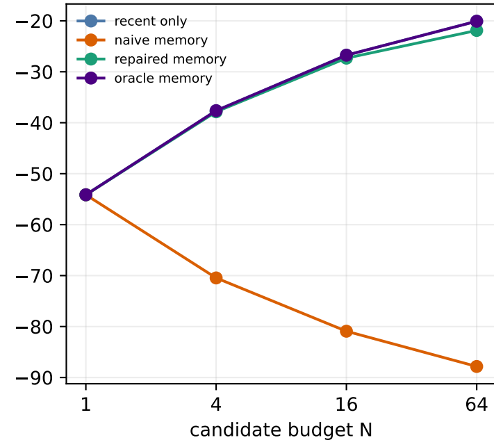
Taxi-v3
