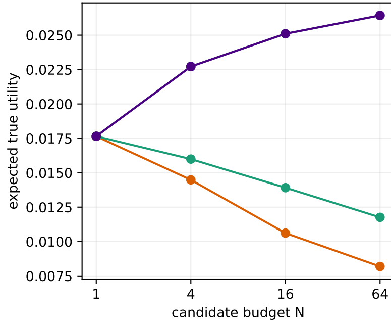
FrozenLake-v1
